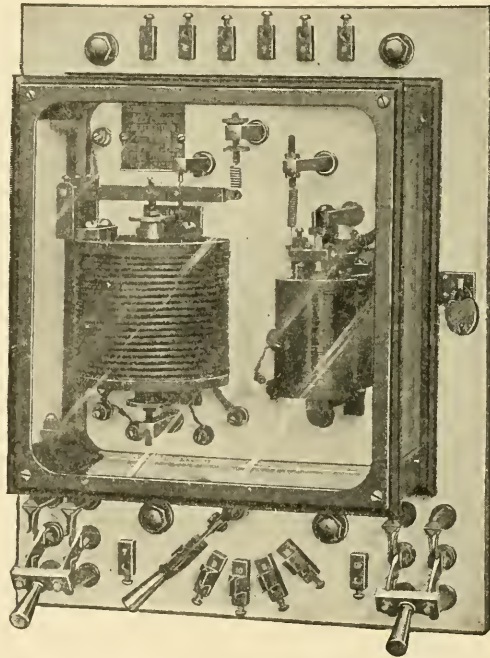
Fig. 16. Tirrill Regulator for Operating Directly on Generator Field
